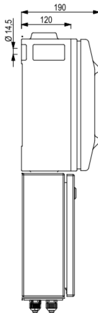
Fig. 2 Side view
